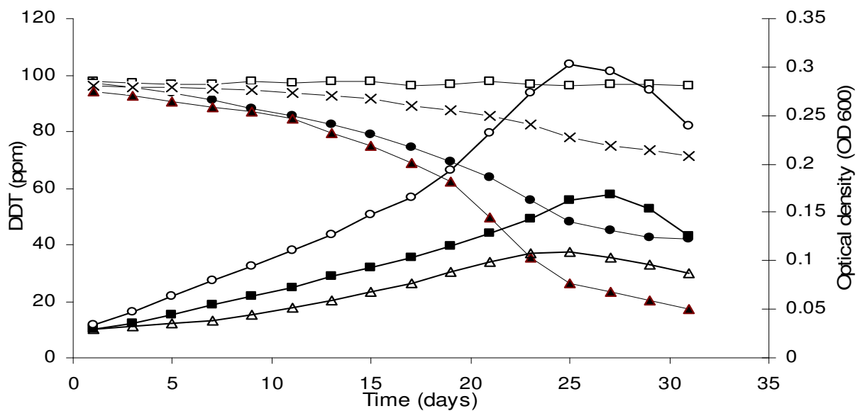
Figure 6. Bacterial growth and DDT degradation. Results are means where n=2 and SE < 5\% of means in all cases. The symbols represents: \square - Control, \Delta - growth curve for isolate 110, \blacksquare - growth curve for isolate 102, \circ - growth curve for the six mixed isolates, \times -DDT degradation curve for isolate 110, \bullet -DDT degradation curve for isolate 102, \blacktriangle - DDT degradation curve for the six mixed isolates.
